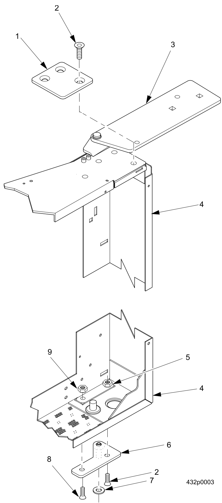
FIGURE 2: DOOR HINGE ASSEMBLIES
